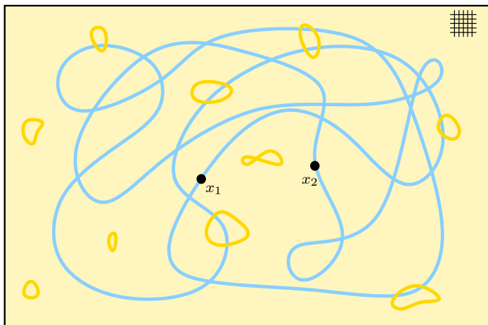
FIGURE 5. Illustration for loop correlations between distant points. In order to belong to the same loop, they must belong to long loops, and also to the same partition element.
