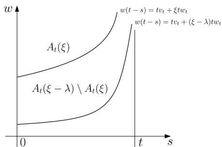
FIG. 2. Intuition behind (4.35).
